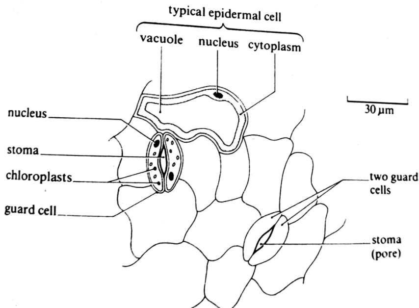
Structure of the stomata
