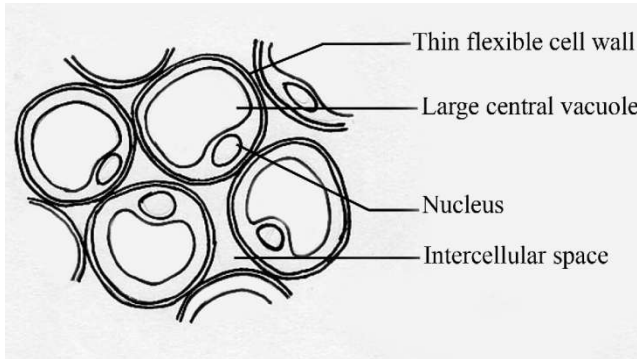
Diagram of general parenchyma cells
