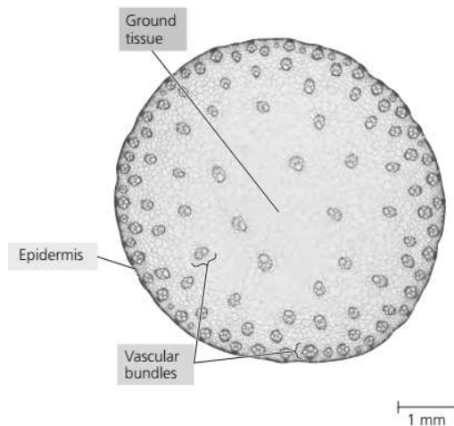
(Figure cross section of typical monocot stem)
