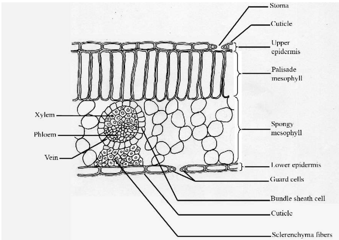
T.S of typical Dicot Leaf
