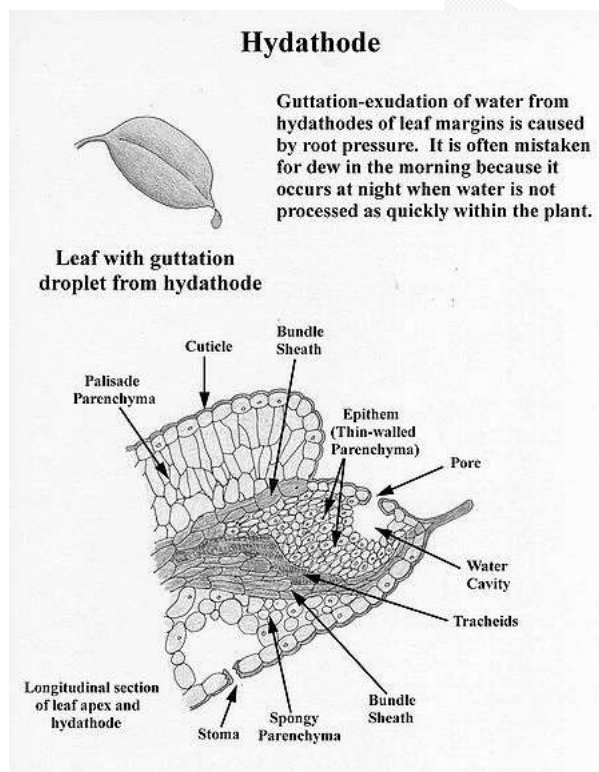
Fig 7.3: structure of a hydathode
