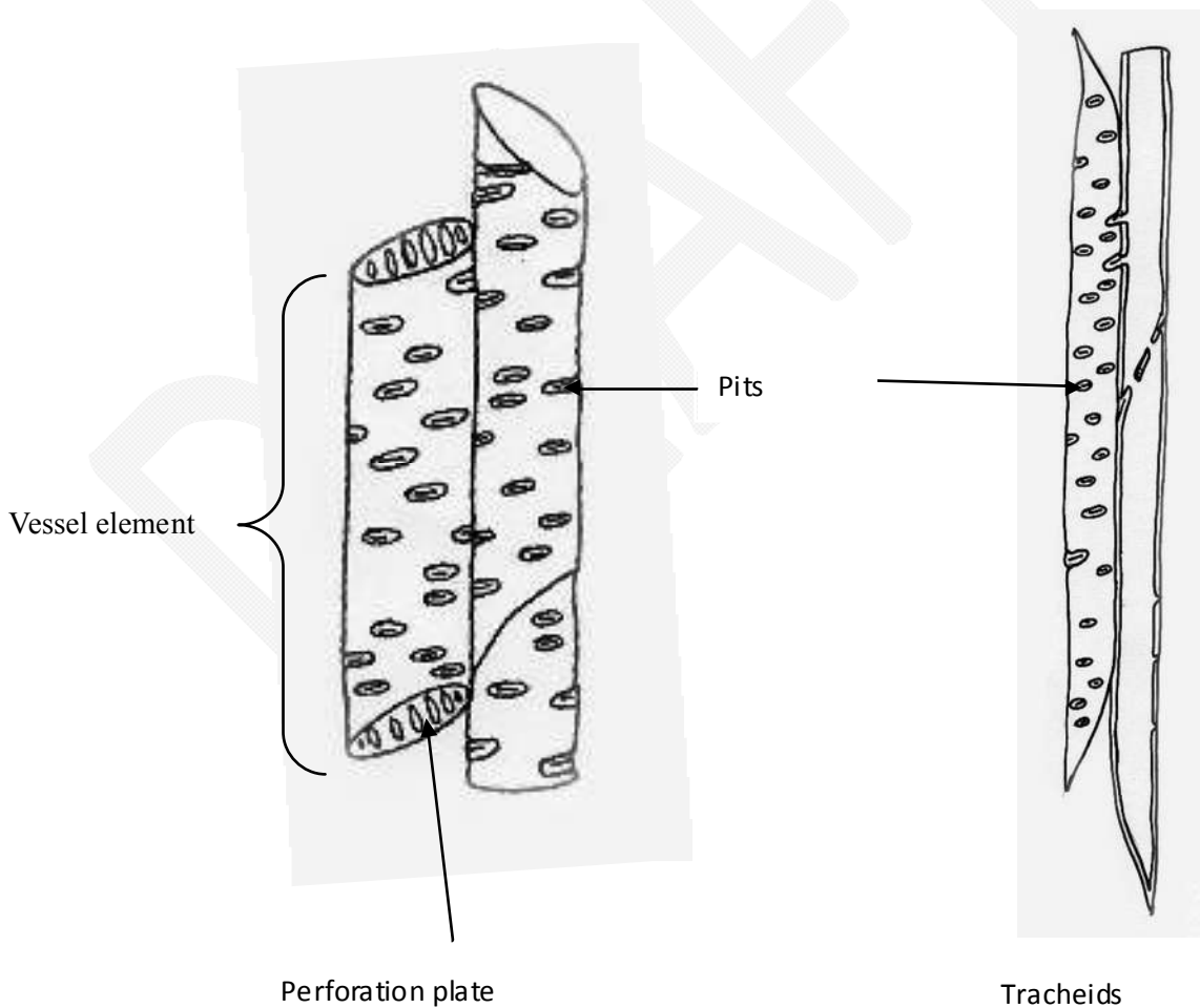
Vessel elements with perforation plate
