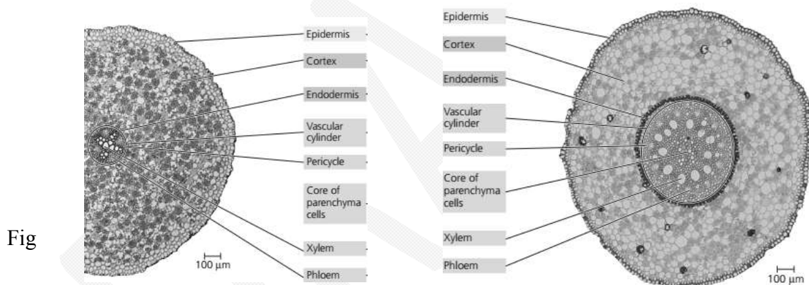
Fig Primary structure of typical Dicot Primary structure of typical monocot root
